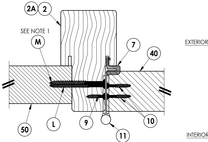
4 7 HORIZONTAL CROSS SECTION Inswing shown (Outswing similar)
