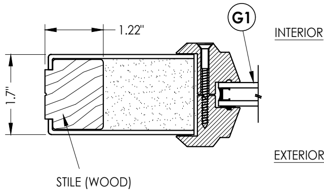
1 HORIZONTAL CROSS SECTION
