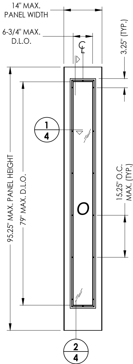
40 SIDELITE PANEL Therma-Tru Fiberglass
