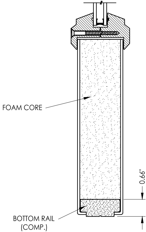
2 VERTICAL CROSS SECTION
